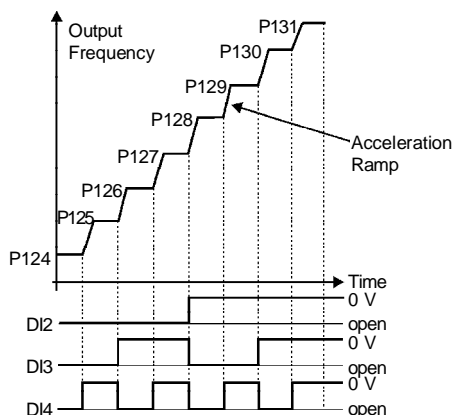
Figure 6.5 - Time Diagram of the multispeed function
