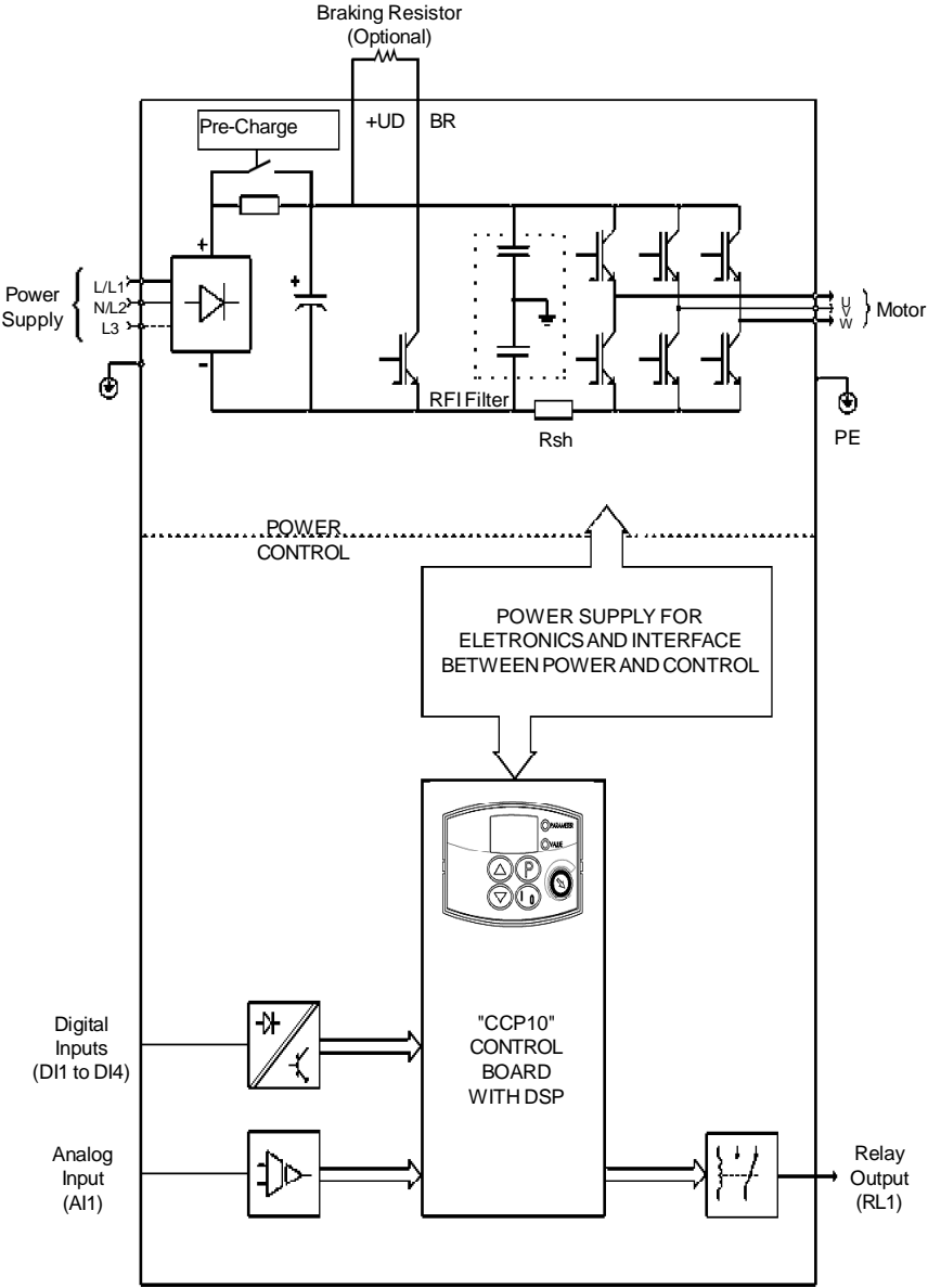
Figure 2.2 - CFW-10 Block Diagram for model 7.3 A and 10.0 A/200-240 V (single-phase) and 10.0 A and 15.2 A/200-240 V (three-phase)
