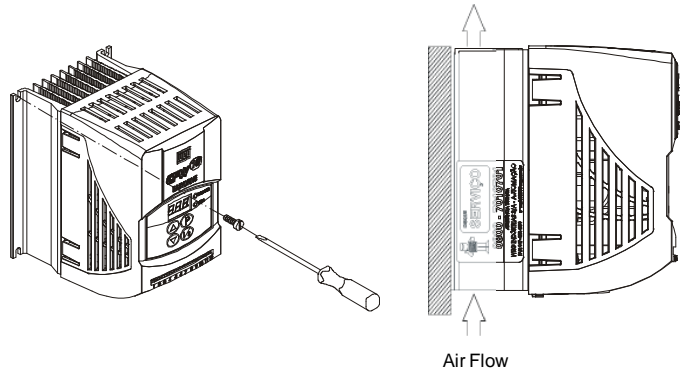
Figure 3.3 - Mounting Procedures for the CFW-10
