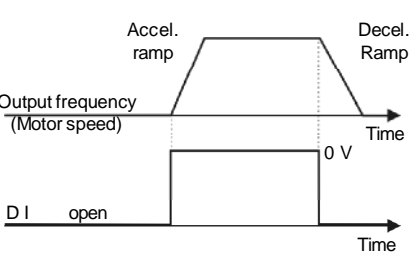
b) START/STOP
