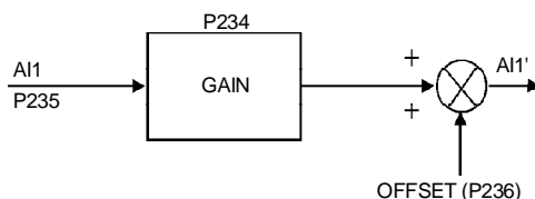
Figure 6.18 b) - Block diagram of the analog input AI
